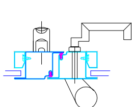
GACHE ELECTRIQUE + SERR 1Pt BEQUILLE INT. BATON EXT CREMONE POMPIER
